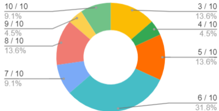
25-35 vs. Score
