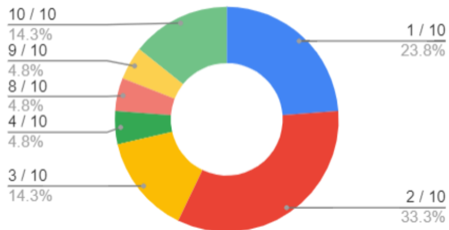
35-40 vs. Score
