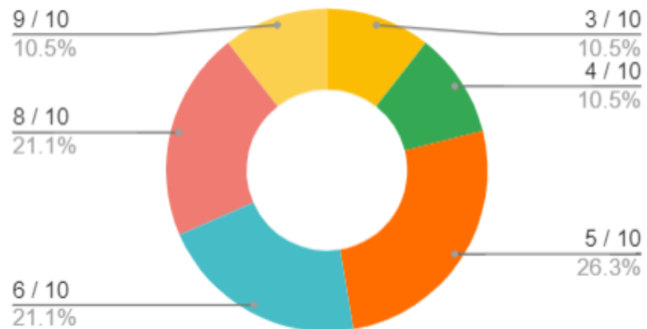
18-25 vs. Score
